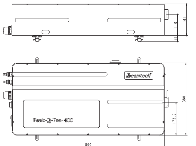
Peak-Q-Pro-200/400 激光头
