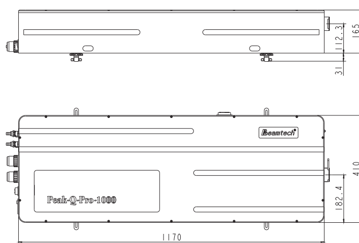
Peak-Q-Pro-1000 激光头
