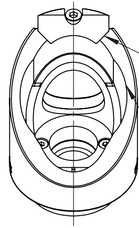
VIEW A-A ROTATED 45°
