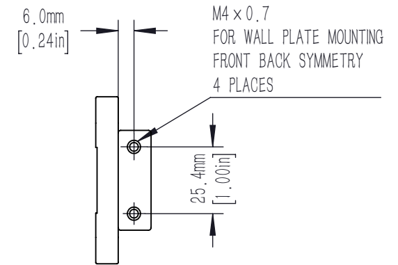
VIEW B
