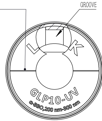
DRAWING OF PARTIAL ENLARGEMENT B SCALE 2:1
