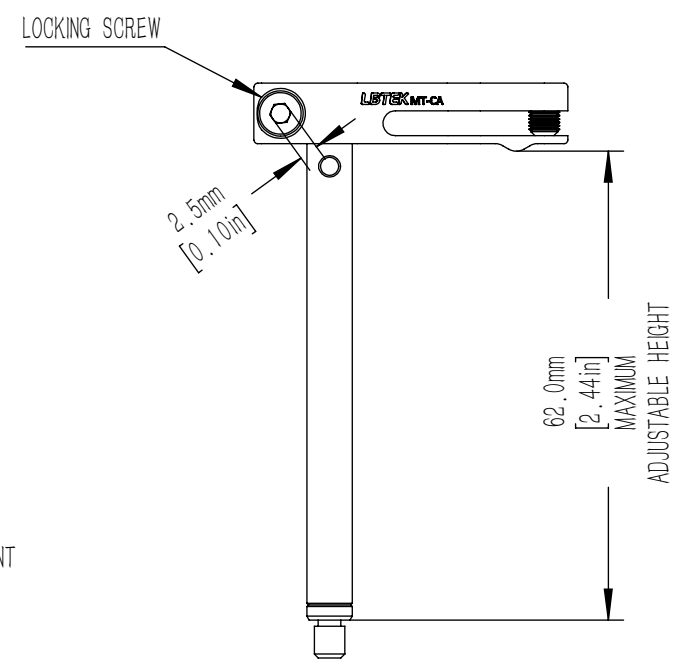
AUXILIARY VIEW
